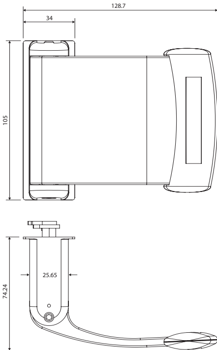
Shown at rest. Paddle travel: 50.8mm.
